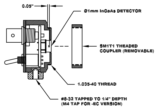
CROSS SECTION VIEW X-X
